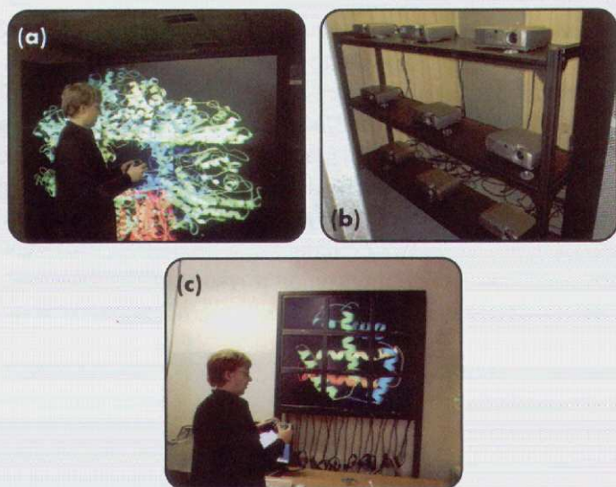
Figure 3: (a) and (b) Tiled 3x3 Projector Display with 9 projectors, (c) Tiled 3x3 LC Display.
