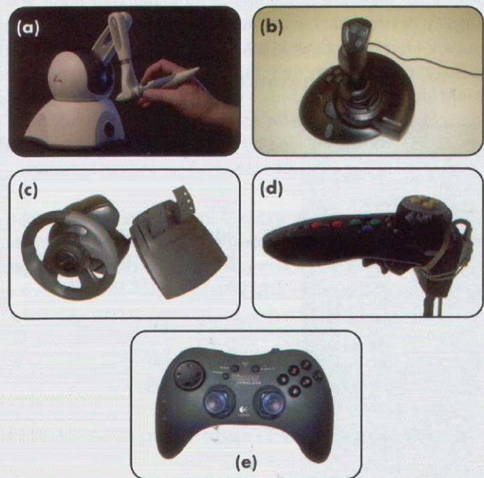
Figure 1: (a) The PHANTOM Omni device by SensAble Technologies, Inc.; (b) Microsoft SideWinder Force Feedback Pro Joystick; (c) Microsoft SideWinder Force Feedback Wheel; (d) modified Nintendo64 controller; (e) the Logitech® WingMan® Cordless Rumblepad.
