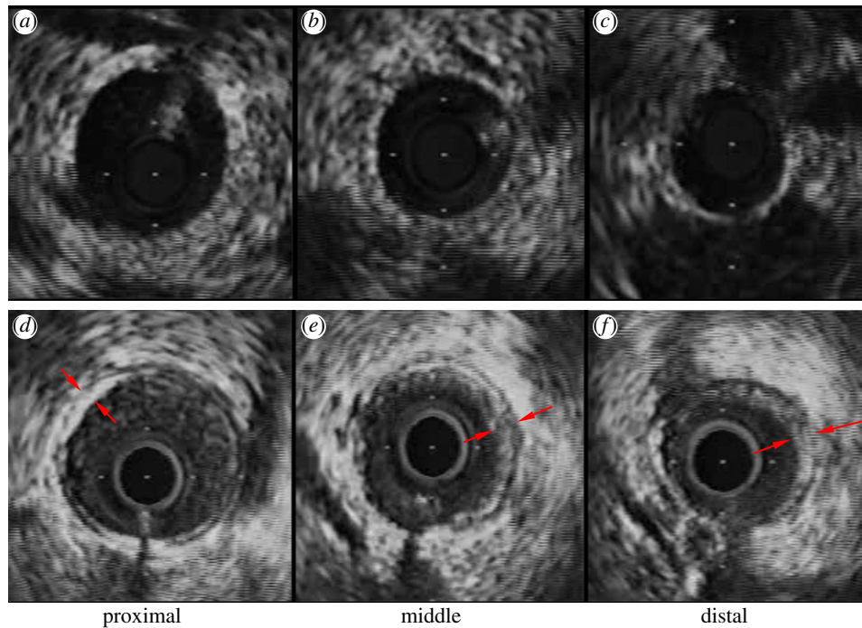
Figure 1. IVUS measurements at (a,d) proximal, (b,e) middle and (c,f) distal sites along the main trunk of the LAD artery for (a–c) control and (d–f) high-fat diet. Arrows refer to the plaques. (Online version colour.)
